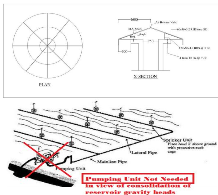
Fig; The Improved Intake Canopy for Sprinkler/Drip Specific Distribution System
